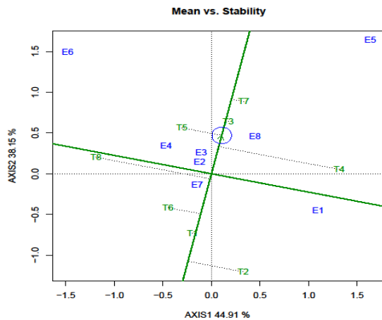
Figure (5): GGE biplot visualization of the genotypes ranking for both yield and stability performance over environments. Where, E1=Dedo 2020, E2= Gechi 2020, E3= Dedo 2021, E4= Gechi 2021, E5= Yem 2021, E6= Dedo 2022, E7= Gechi 2022 and E8= Yem 2022 and T1= Dafo, T2= Guta, T3= Biftu, T4= Abdane, T5= HB1307, T6= Harbu, T7= Robera and T8= Adoshe
