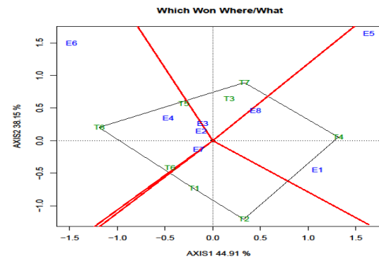
Figure (2): The polygon view of GGE biplot to the identification of winning genotypes and their related Mega environments: Where, E1=Dedo 2020, E2= Gechi 2020, E3= Dedo 2021, E4= Gechi 2021, E5= Yem 2021, E6= Dedo 2022, E7= Gechi 2022 and E8= Yem 2022 and T1= Dafo, T2= Guta, T3= Biftu, T4= Abdane, T5= HB1307, T6= Harbu, T7= Robera and T8= Adoshe
