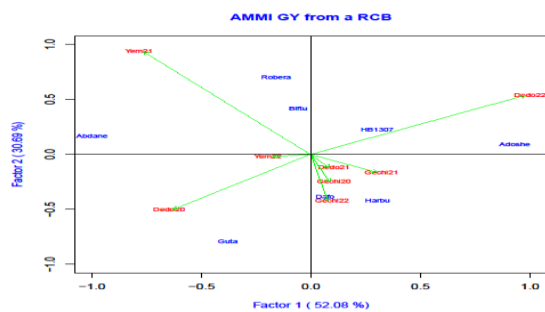
Figure (1): Biplot of interaction principal component axis (IPCA1) against interaction principal component axis (IPCA2) food barley varieties evaluated across eight environments of southwestern Ethiopia
