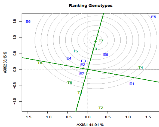
Figure (3): GGE biplot of ideal genotypes and comparison of the genotypes with respect to the ideal genotype:Where,E1=Dedo 2020,E2= Gechi 2020,E3= Dedo 2021,E4= Gechi 2021,E5= Yem 2021,E6= Dedo 2022,E7= Gechi 2022 and E8= Yem 2022 and T1= Dafo,T2= Guta,T3= Biftu,T4= Abdane,T5= HB1307,T6= Harbu,T7= Robera and T8= Adoshe
