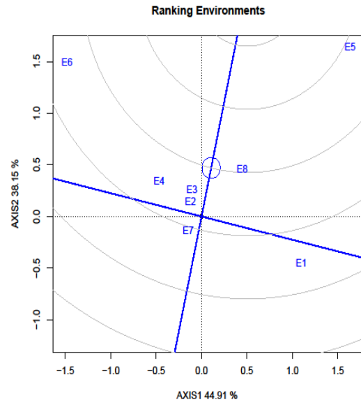
Figure (4): GGE biplot of ideal environments and comparison of the environments with respect to the ideal environment:E1=Dedo 2020,E2= Gechi 2020,E3= Dedo 2021,E4= Gechi 2021,E5= Yem 2021,E6= Dedo 2022,E7= Gechi 2022 and E8= Yem 2022
